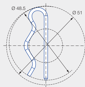
Dimensions of the slip-on connection top view
